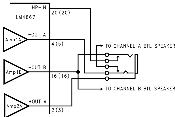
Figure 46. Headphone Circuit
